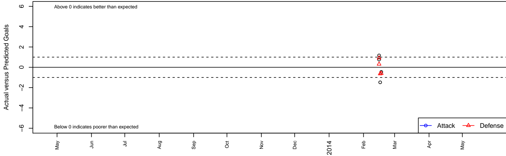
Pride SC 01 Predators G00 Dots are actual minus expected GF (blue circles) and GA (red triangles). Blue line is smoothed change in attack strength. Red is smoothed change in defense strength.
